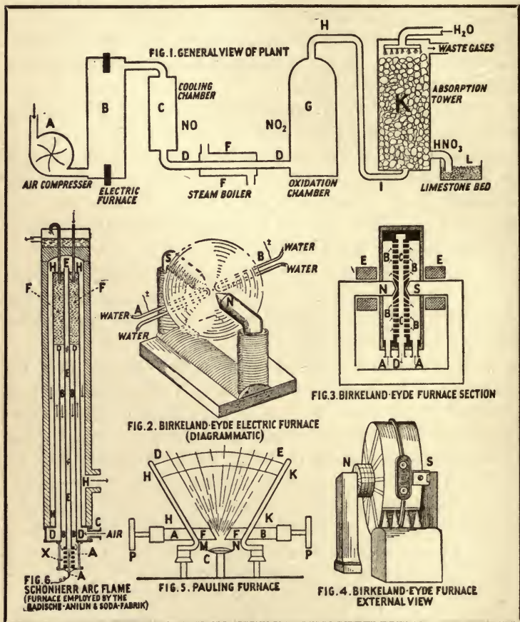
FIG. 2.—Nitric acid from the atmosphere.
